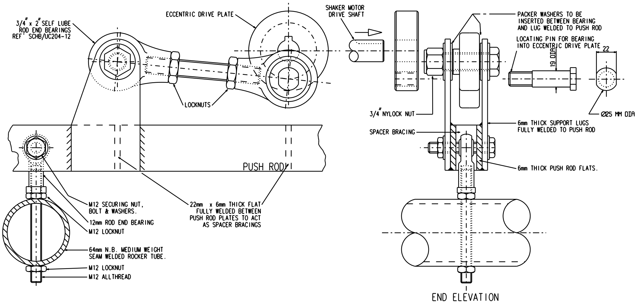
SECTIONAL DETAIL OF SHAKER MECHANISM ASSEMBLY ON TUBE FILTER UNITS
