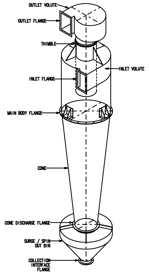
GENERAL COMPONENTS OF DUSTAIR CYCLONE
